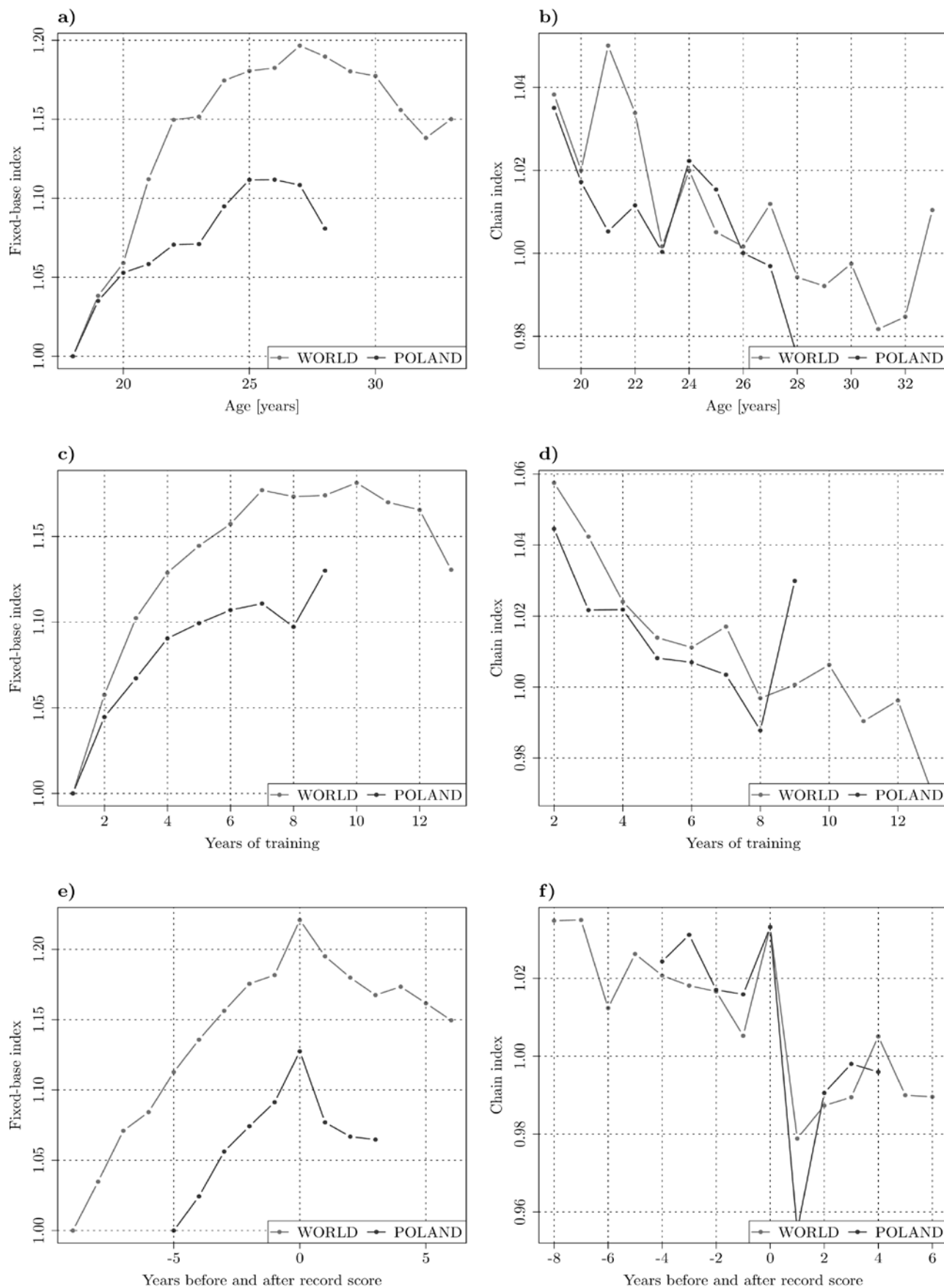
Figure 2. Fixed-base indices (a, c, and e) and chain indices (b, d, and f) obtained for the three protocols
